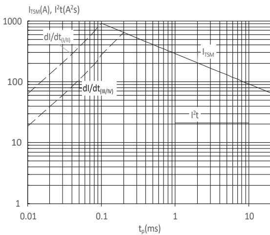
FIG : Non-repetitive surge peak on-state current for a sinusoidal pulse with width t_p < 20ms , and corresponding value of I^2t ( I - II : dl/dt < 80A/\mu s ; III-IV : dl/dt < 40A/\mu s )
