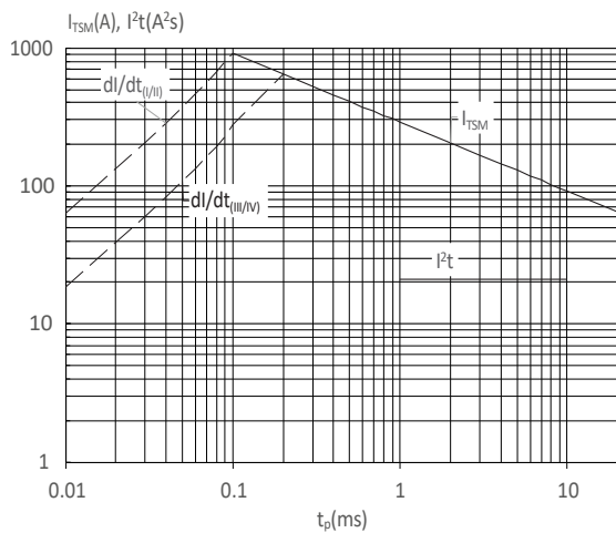
FIG : Non-repetitive surge peak on-state current for a sinusoidal pulse with width t_p < 20ms , and corresponding value of I^2t ( I - II : di/dt < 100A/μs ; III-IV : di/dt < 50A/μs )
