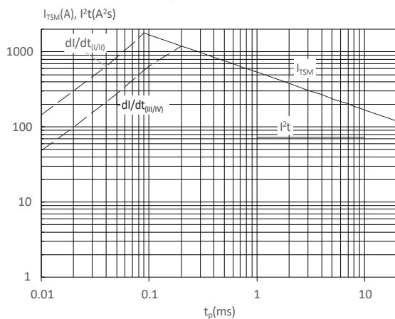
FIG : Non-repetitive surge peak on-state current for a sinusoidal pulse with width t_p < 20\text{ms} , and corresponding value of I^2t ( I - II : dl/dt < 100\text{A}/\mu\text{s} ; III-IV : dl/dt < 50\text{A}/\mu\text{s} )
