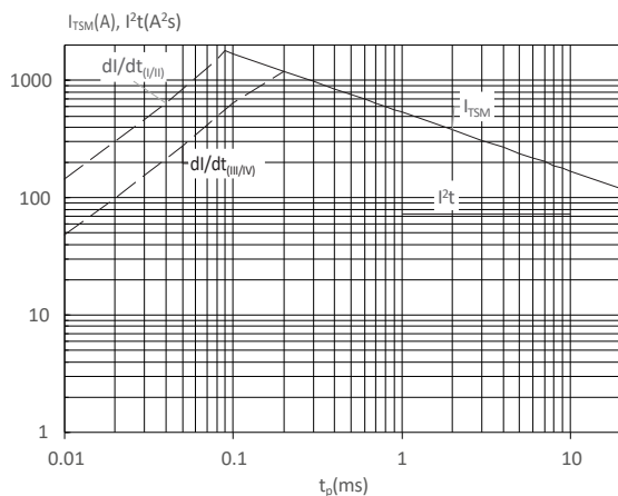
FIG : Non-repetitive surge peak on-state current for a sinusoidal pulse with width t_p < 20\text{ms} , and corresponding value of I^2t ( I - II : dl/dt < 80\text{A}/\mu\text{s} ; III-IV : dl/dt < 40\text{A}/\mu\text{s} )
