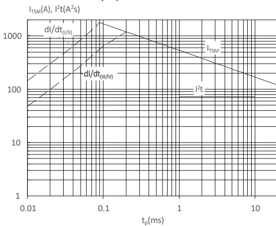
FIG : Non-repetitive surge peak on-state current for a sinusoidal pulse with width t_p < 20\text{ms} , and corresponding value of I^2t ( I - II : di/dt < 80\text{A}/\mu\text{s} ; III-IV : di/dt < 40\text{A}/\mu\text{s} )
