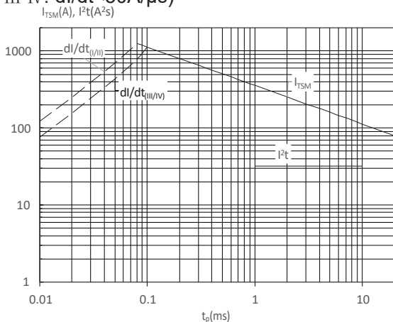
FIG : Non-repetitive surge peak on-state current for a sinusoidal pulse with width t_p < 20ms , and corresponding value of I^2t (I - II: dl/dt < 100A/\mu s ; III-IV: dl/dt < 50A/\mu s )
