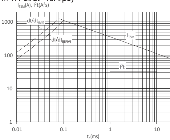
FIG : Non-repetitive surge peak on-state current for a sinusoidal pulse with width t_p < 20\text{ms} , and corresponding value of I^2t (I - II: di/dt < 80\text{A}/\mu\text{s} ; III-IV: di/dt < 40\text{A}/\mu\text{s} )
