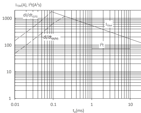
FIG : Non-repetitive surge peak on-state current for a sinusoidal pulse with width t_p < 20ms , and corresponding value of I^2t ( I - II : dl/dt < 80A/\mu s ; III-IV : dl/dt < 40A/\mu s )
