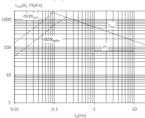
FIG : Non-repetitive surge peak on-state current for a sinusoidal pulse with width t_p < 20\text{ms} , and corresponding value of I^2t ( I -II : dl/dt < 100\text{A}/\mu\text{s} ; III-IV : dl/dt < 50\text{A}/\mu\text{s} )
