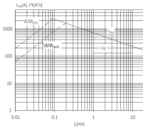
FIG : Non-repetitive surge peak on-state current for a sinusoidal pulse with width t_p < 20\text{ms} , and corresponding value of I^2t ( I - II : di/dt < 80\text{A}/\mu\text{s} ; III-IV : di/dt < 40\text{A}/\mu\text{s} )
