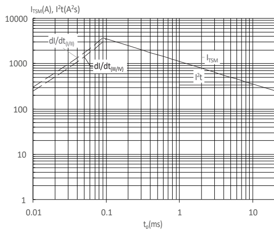
FIG : Non-repetitive surge peak on-state current for a sinusoidal pulse with width t_p < 20ms , and corresponding value of I^2t (I - II: di/dt < 100A/\mu s ; III-IV: di/dt < 50A/\mu s )
