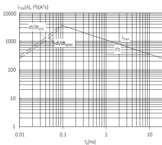
FIG : Non-repetitive surge peak on-state current for a sinusoidal pulse with width t_p < 20\text{ms} , and corresponding value of I^2t ( I - II: di/dt < 100\text{A}/\mu\text{s} ; III-IV: di/dt < 50\text{A}/\mu\text{s} )
