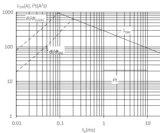
FIG : Non-repetitive surge peak on-state current for a sinusoidal pulse with width t_p < 20\text{ms} , and corresponding value of I^2t ( I - II -III: dl/dt < 50\text{A}/\mu\text{s} ; IV: dl/dt < 20\text{A}/\mu\text{s} )
