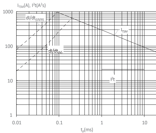
FIG : Non-repetitive surge peak on-state current for a sinusoidal pulse with width t_p < 20\text{ms} , and corresponding value of I^2t ( I - II -III: dl/dt < 80\text{A}/\mu\text{s} ; IV: dl/dt < 40\text{A}/\mu\text{s} )
