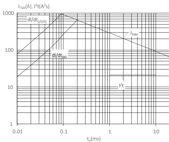
FIG : Non-repetitive surge peak on-state current for a sinusoidal pulse with width t_p < 20\text{ms} , and corresponding value of I^2t (I - II -III: dl/dt < 100\text{A}/\mu\text{s} ; IV: dl/dt < 50\text{A}/\mu\text{s} )
