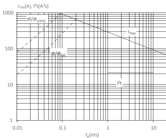
FIG : Non-repetitive surge peak on-state current for a sinusoidal pulse with width t_p < 20\text{ms} , and corresponding value of I^2t ( I -II -III: dl/dt < 100\text{A}/\mu\text{s} ; IV: dl/dt < 50\text{A}/\mu\text{s} )
