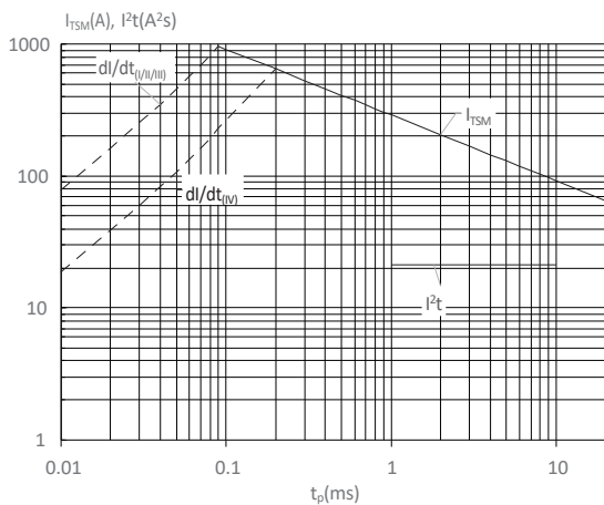
FIG : Non-repetitive surge peak on-state current for a sinusoidal pulse with width t_p < 20ms , and corresponding value of I^2t ( I - II -III: dl/dt < 80A/\mu s ; IV: dl/dt < 40A/\mu s )
