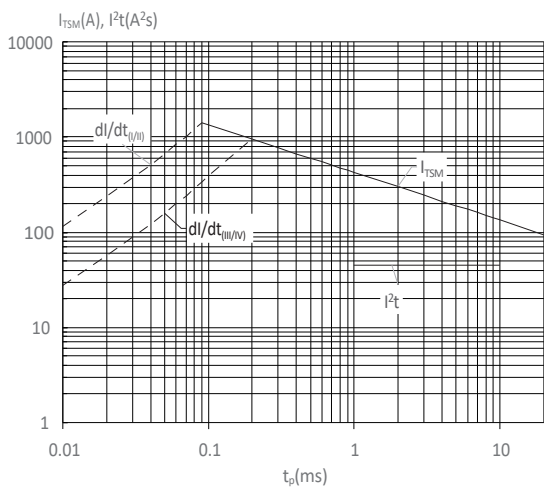
FIG : Non-repetitive surge peak on-state current for a sinusoidal pulse with width t_p < 20\text{ms} , and corresponding value of I^2t ( I - II : di/dt < 50\text{A}/\mu\text{s} ; III-IV : di/dt < 20\text{A}/\mu\text{s} )
