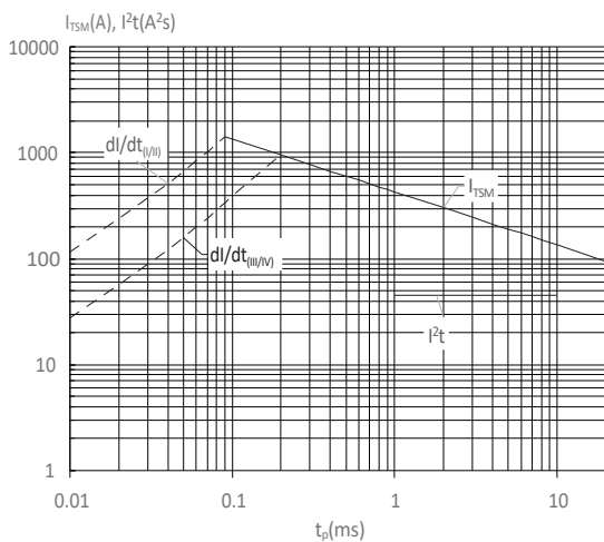
FIG : Non-repetitive surge peak on-state current for a sinusoidal pulse with width t_p < 20\text{ms} , and corresponding value of I^2t ( I - II : dl/dt < 100\text{A}/\mu\text{s} ; III-IV : dl/dt < 70\text{A}/\mu\text{s} )
