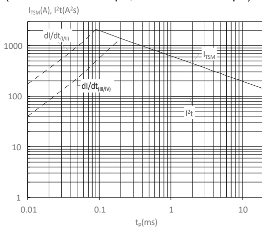
FIG : Non-repetitive surge peak on-state current for a sinusoidal pulse with width t_p < 20ms , and corresponding value of I^2t ( I - II : di/dt < 100A/\mu s ; III-IV : di/dt < 70A/\mu s )
