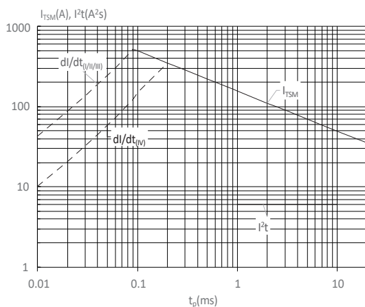
FIG : Non-repetitive surge peak on-state current for a sinusoidal pulse with width t_p < 20\text{ms} , and corresponding value of I^2t ( I - II - III: di/dt < 80\text{A}/\mu\text{s} ; IV: di/dt < 40\text{A}/\mu\text{s} )
