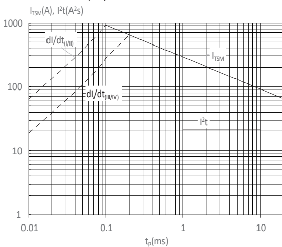
FIG : Non-repetitive surge peak on-state current for a sinusoidal pulse with width t_p < 20\text{ms} , and corresponding value of I^2t ( I - II: di/dt < 80\text{A}/\mu\text{s} ; III-IV: di/dt < 40\text{A}/\mu\text{s} )
