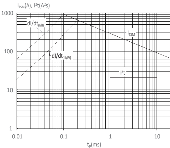
FIG : Non-repetitive surge peak on-state current for a sinusoidal pulse with width t_p < 20\text{ms} , and corresponding value of I^2t ( I - II : di/dt < 100\text{A}/\mu\text{s} ; III-IV : di/dt < 50\text{A}/\mu\text{s} )
