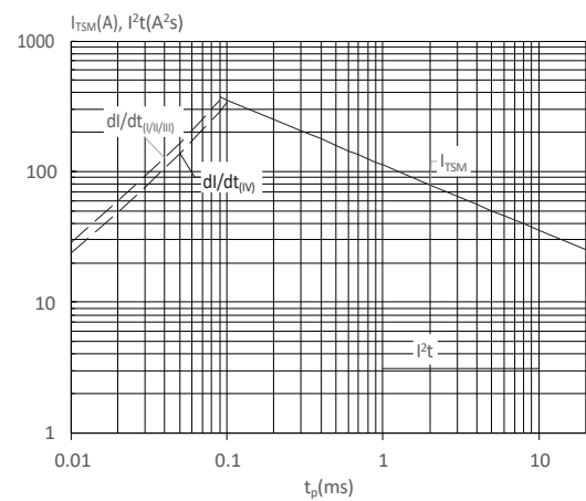
FIG : Non-repetitive surge peak on-state current for a sinusoidal pulse with width t_p < 20\text{ms} , and corresponding value of I^2t (I - II - III: di/dt < 70\text{A}/\mu\text{s} ; IV: di/dt < 40\text{A}/\mu\text{s} )
