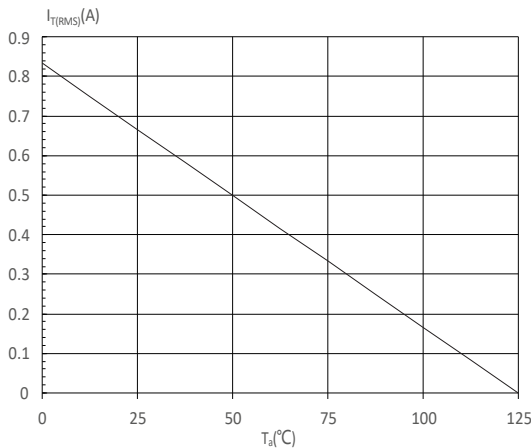
FIG : On-state characteristics
