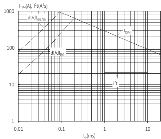
FIG : Non-repetitive surge peak on-state current for a sinusoidal pulse with width t_p < 20\text{ms} , and corresponding value of I^2t (I - II - III: dl/dt < 50\text{A}/\mu\text{s} ; IV: dl/dt < 20\text{A}/\mu\text{s} )
