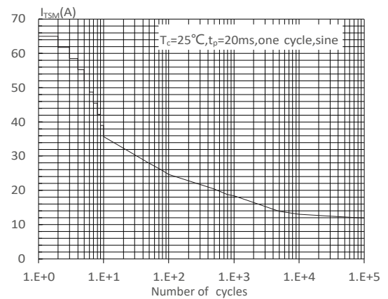
FIG : Non-repetitive surge peak on-state current for a sinusoidal pulse with width t_p < 20\text{ms} , and corresponding value of I^2t ( I - II -III: dl/dt < 80\text{A}/\mu\text{s} ; IV: dl/dt < 40\text{A}/\mu\text{s} )
