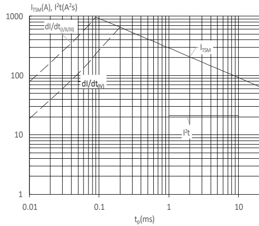
FIG : Non-repetitive surge peak on-state current for a sinusoidal pulse with width t_p < 20ms , and corresponding value of I^2t (I - II - III: dl/dt < 100A/\mu s ; IV: dl/dt < 50A/\mu s )
