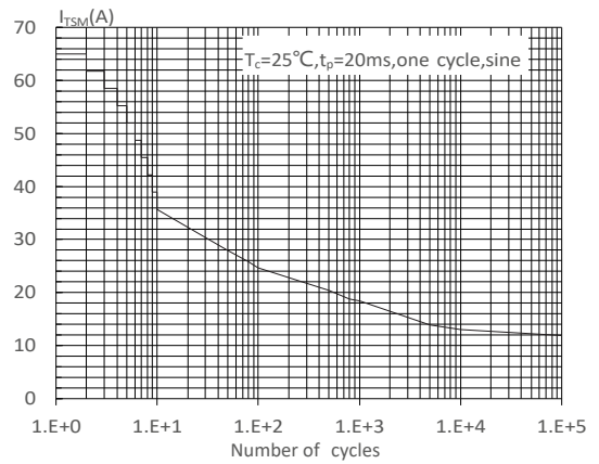
FIG : Non-repetitive surge peak on-state current for a sinusoidal pulse with width t_p < 20ms , and corresponding value of I^2t (I - II - III: dl/dt < 100A/\mu s ; IV: dl/dt < 50A/\mu s )
