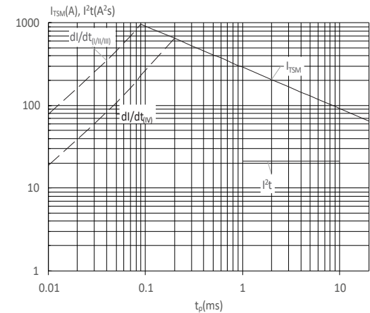
FIG : Non-repetitive surge peak on-state current for a sinusoidal pulse with width t_p < 20\text{ms} , and corresponding value of I^2t ( I - II - III: di/dt < 100\text{A}/\mu\text{s} ; IV: di/dt < 50\text{A}/\mu\text{s} )
