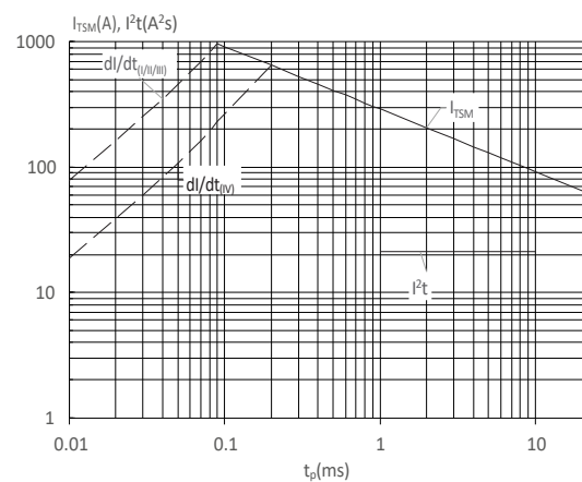
FIG : Non-repetitive surge peak on-state current for a sinusoidal pulse with width t_p < 20\text{ms} , and corresponding value of I^2t ( I - II -III: dl/dt < 100\text{A}/\mu\text{s} ; IV: dl/dt < 50\text{A}/\mu\text{s} )
