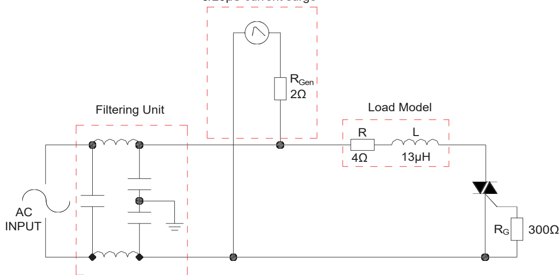
IEC61000-4-5 Standards Surge Generator 1.2/50 \mu S voltage surge 8/20 \mu S current surge
