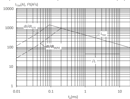
FIG : Non-repetitive surge peak on-state current for a sinusoidal pulse with width t_p < 20\text{ms} , and corresponding value of I^2t ( I - II : di/dt < 80\text{A}/\mu\text{s} ; III-IV : di/dt < 50\text{A}/\mu\text{s} )
