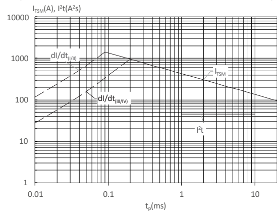
FIG : Non-repetitive surge peak on-state current for a sinusoidal pulse with width t_p < 20ms , and corresponding value of I^2t ( I - II : di/dt < 100A/\mu s ; III-IV : di/dt < 70A/\mu s )
