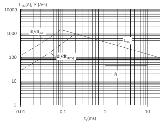
FIG : Non-repetitive surge peak on-state current for a sinusoidal pulse with width t_p < 20ms , and corresponding value of I^2t ( I - II : di/dt < 80A/\mu s ; III-IV : di/dt < 50A/\mu s )
