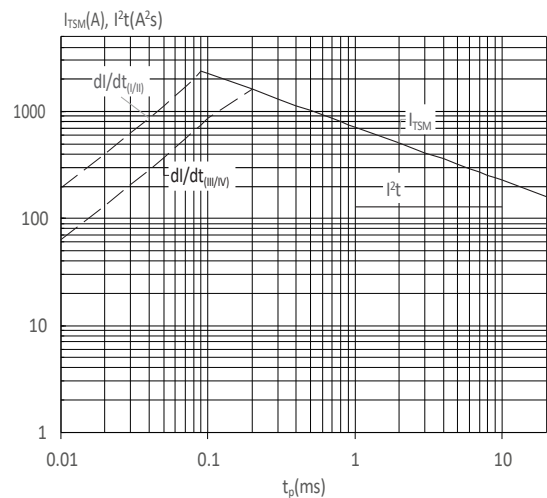
FIG : Non-repetitive surge peak on-state current for a sinusoidal pulse with width t_p < 20\text{ms} , and corresponding value of I^2t (I - II : dl/dt < 100\text{A}/\mu\text{s} ; III-IV : dl/dt < 50\text{A}/\mu\text{s} )
