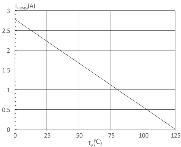
FIG : On-state characteristics
