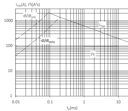
FIG : Non-repetitive surge peak on-state current for a sinusoidal pulse with width t_p < 20\text{ms} , and corresponding value of I^2t (I - II: di/dt < 100\text{A}/\mu\text{s} ; III-IV: di/dt < 70\text{A}/\mu\text{s} )
