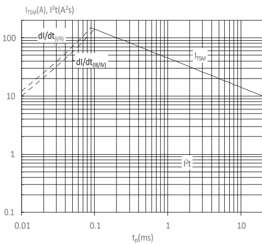
FIG : Non-repetitive surge peak on-state current for a sinusoidal pulse with width t_p < 20\text{ms} , and corresponding value of I^2t (I - II : di/dt < 50\text{A}/\mu\text{s} ; III-IV : di/dt < 30\text{A}/\mu\text{s} )
