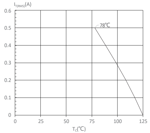
FIG : On-state characteristics
