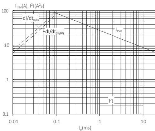
FIG : Non-repetitive surge peak on-state current for a sinusoidal pulse with width t_p < 20\text{ms} , and corresponding value of I^2t (I - II : di/dt < 50\text{A}/\mu\text{s} ; III-IV : di/dt < 20\text{A}/\mu\text{s} )
