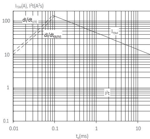
FIG : Non-repetitive surge peak on-state current for a sinusoidal pulse with width t_p < 20\text{ms} , and corresponding value of I^2t ( I - II : di/dt < 30\text{A}/\mu\text{s} ; III-IV : di/dt < 20\text{A}/\mu\text{s} )
