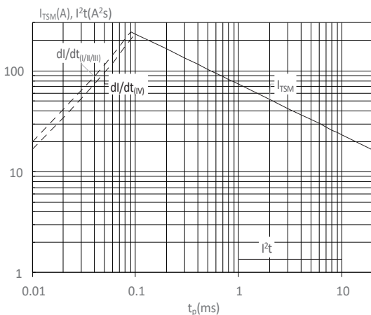
FIG : Non-repetitive surge peak on-state current for a sinusoidal pulse with width t_p < 20\text{ms} , and corresponding value of I^2t (I - II - III: di/dt < 50\text{A}/\mu\text{s} ; IV: di/dt < 30\text{A}/\mu\text{s} )
