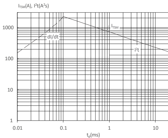
FIG : Non-repetitive surge peak on-state current for a sinusoidal pulse with width t_p < 20\text{ms} , and corresponding value of I^2t ( dl/dt < 100\text{A}/\mu\text{s} )
