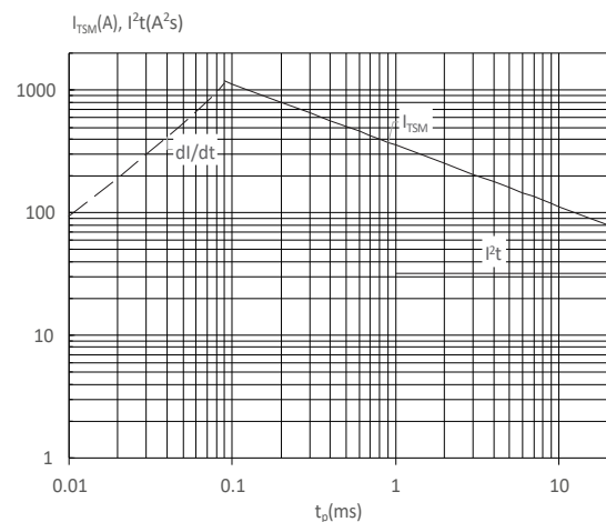
FIG : Non-repetitive surge peak on-state current for a sinusoidal pulse with width t_p < 20ms , and corresponding value of I^2t ( di/dt < 50A/\mu s )
