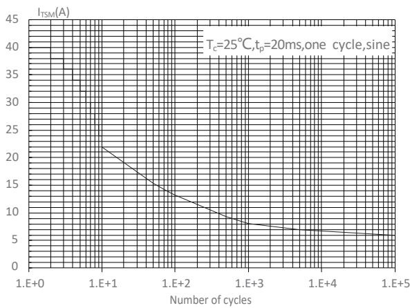
FIG : Non-repetitive surge peak on-state current for a sinusoidal pulse with width t_p < 20\text{ms} , and corresponding value of I^2t ( di/dt < 80\text{A}/\mu\text{s} )
