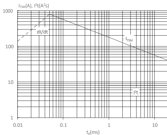
FIG : Non-repetitive surge peak on-state current for a sinusoidal pulse with width t_p < 20\text{ms} , and corresponding value of I^2t ( di/dt < 80\text{A}/\mu\text{s} )
