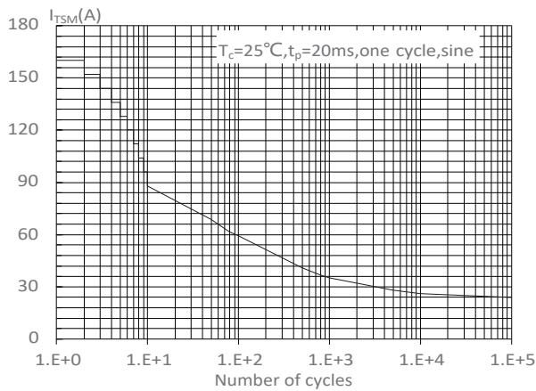
FIG : Non-repetitive surge peak on-state current for a sinusoidal pulse with width t_p < 20ms , and corresponding value of I^2t ( dl/dt < 100A/\mu s )
