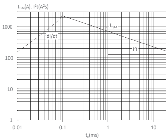
FIG : Non-repetitive surge peak on-state current for a sinusoidal pulse with width t_p < 20ms , and corresponding value of I^2t ( dl/dt < 100A/\mu s )
