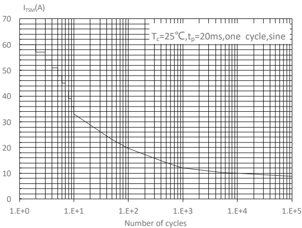
FIG : Non-repetitive surge peak on-state current for a sinusoidal pulse with width t_p < 20ms , and corresponding value of I^2t ( di/dt < 50A/μs )
