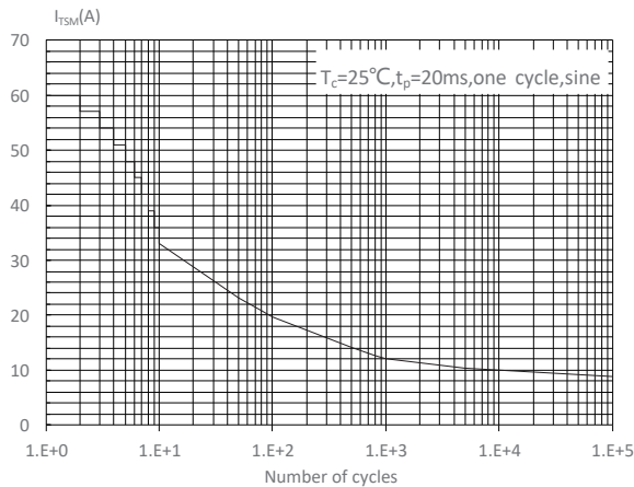
FIG : Non-repetitive surge peak on-state current for a sinusoidal pulse with width t_p < 20ms , and corresponding value of I^2t ( di/dt < 80A/μs )
