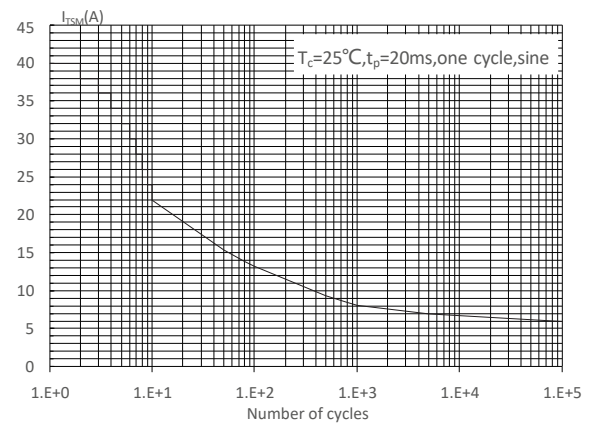
FIG : Non-repetitive surge peak on-state current for a sinusoidal pulse with width t_p < 20ms , and corresponding value of I^2t ( di/dt < 50A/\mu s )
