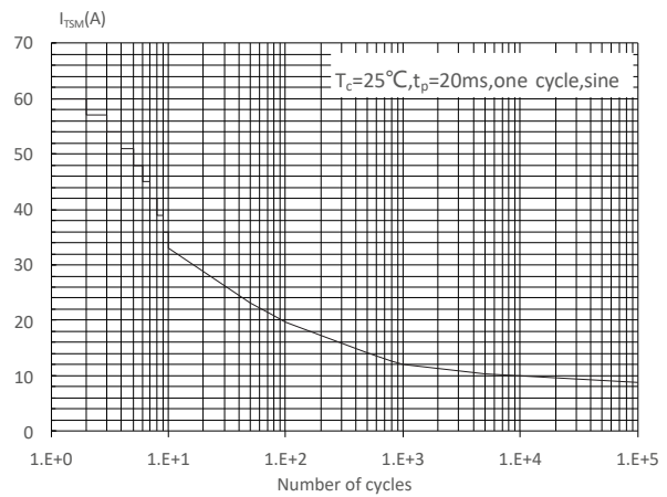
FIG : Non-repetitive surge peak on-state current for a sinusoidal pulse with width t_p < 20\text{ms} , and corresponding value of I^2t ( di/dt < 50\text{A}/\mu\text{s} )
