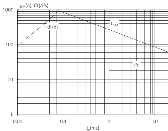
FIG : Non-repetitive surge peak on-state current for a sinusoidal pulse with width t_p < 20\text{ms} , and corresponding value of I^2t ( dI/dt < 80\text{A}/\mu\text{s} )
