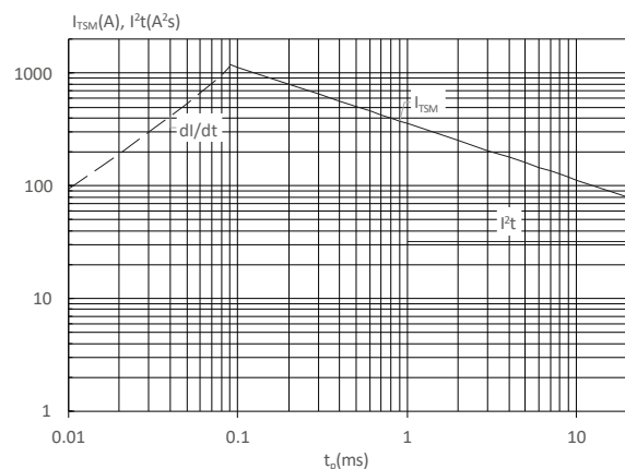
FIG : Non-repetitive surge peak on-state current for a sinusoidal pulse with width t_p < 20ms , and corresponding value of I^2t ( di/dt < 100A/\mu s )
