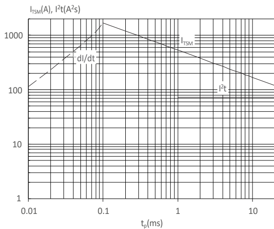
FIG : Non-repetitive surge peak on-state current for a sinusoidal pulse with width t_p < 20\text{ms} , and corresponding value of I^2t ( di/dt < 100\text{A}/\mu\text{s} )
